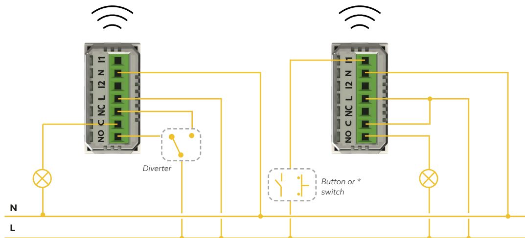
Relè Lite Smart as a diverter.
