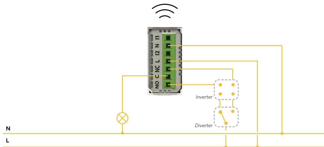
Relè Lite Smart use like an inverter.
