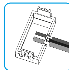
03. Cut, rotate and pull outwards.
